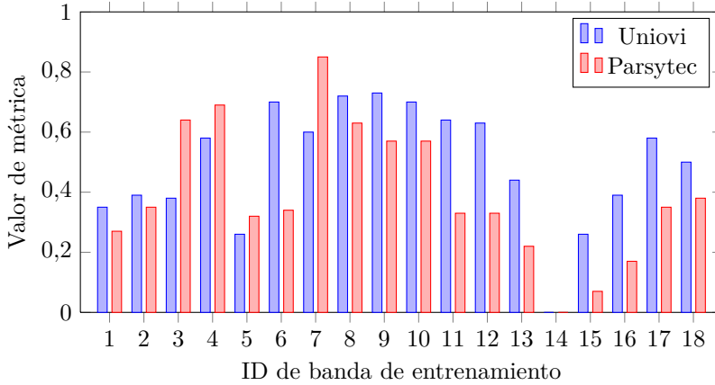
(a) Jaccard
