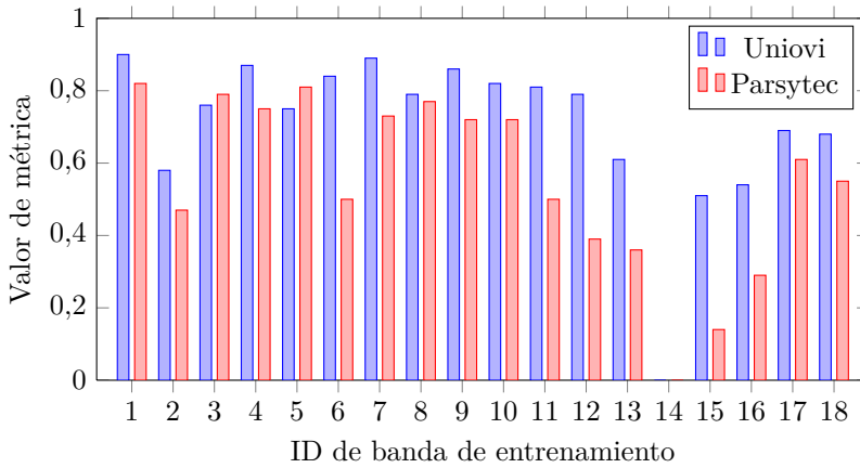
(b) F-Measure
