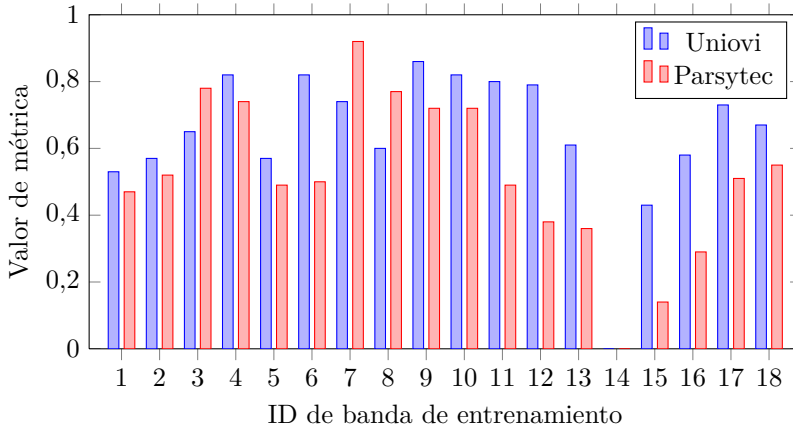
(b) F-Measure
