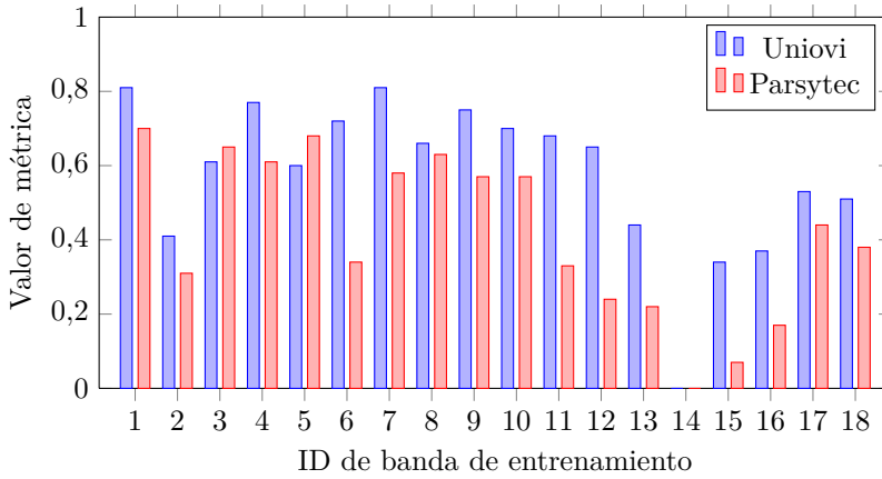
(a) Jaccard
